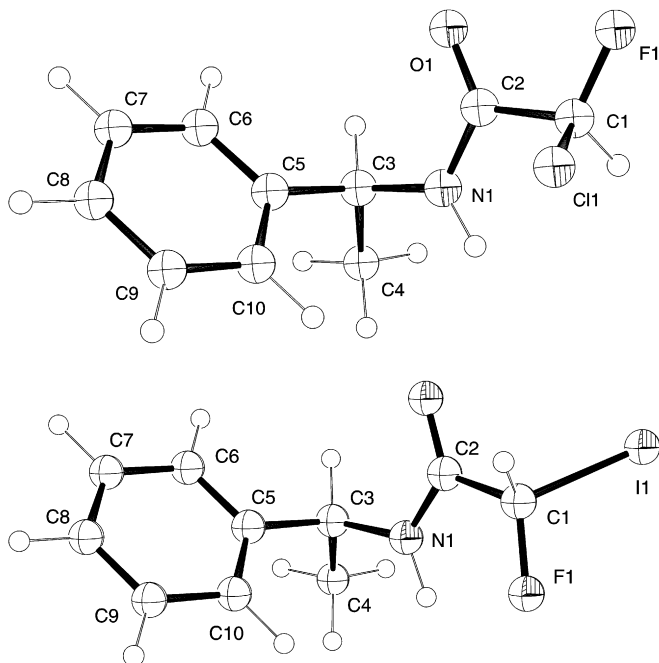
Figure 2. ORTEP view of the less polar diastereoisomers ( 1a above and 3a below) of chlorofluoroethanamide 1 and iodo fluoroethanamide 3 .
