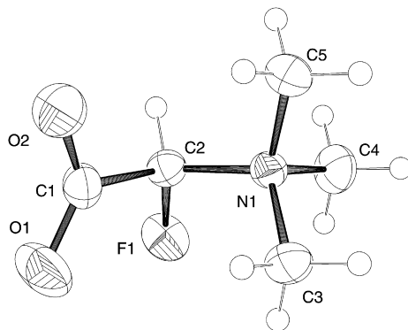
Figure 5. ORTEP view (50% probability ellipsoids) of fluorobetaine 18 .
