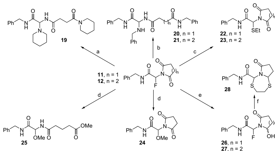
Scheme 4. Reagents and conditions: (a) 15 equiv piperidine, THF, 22 h, rt (89%); (b) 15 equiv \text{BnNH}_2 , THF, rt [20, 24 h (80%); 21, 106 h (62%)]; (c) 1.04 equiv \text{EtSNa} , DMF, rt, 24 h [22, 24 h (51%); 23, 170 h (28%)]; (d) 1 equiv \text{NaOMe} , MeOH, rt, 0.1 h [24 (77%); 25 (76%)]; (e) \text{LiBH}_4 , THF, -15^\circ\text{C} , 4–8 h [26 (59%); 27 (37%)]; (f) \text{HS}(\text{CH}_2)_2\text{SH} , \text{BF}_3 \cdot \text{OEt}_2 , \text{CHCl}_3 , 0^\circ\text{C} , 3.5 h (56%).
